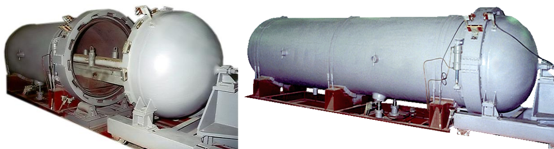
KVG-8 detonation chamber (semi-open/closed positions)
