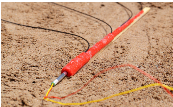
Detonation velocity measurement using Perforated Fiber Probe.
