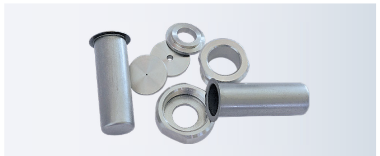
Koenen Steel Shell Tester – test tubes and closing parts
